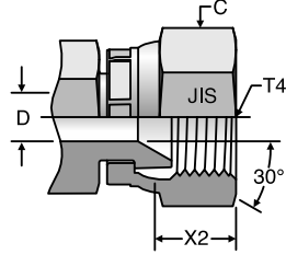
JIS Swivel for 30° Flare
