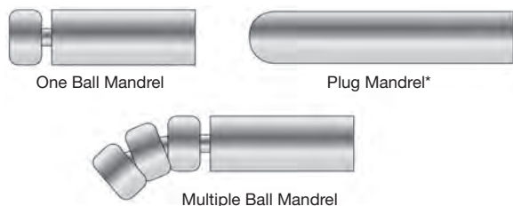
Fig. R60 — Types of mandrels
