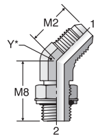
Y* – Across wrench flats
