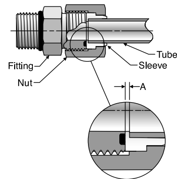
Fig. R23 – Tube length allowance
