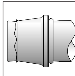
Fig. R40 – Over-set ferrule
