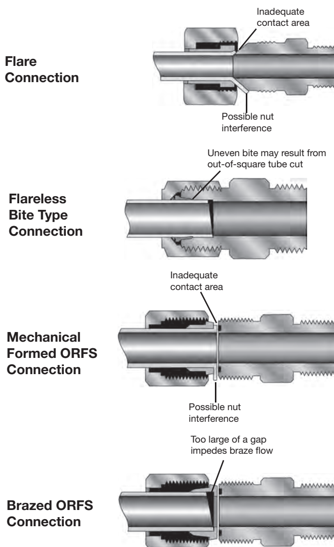
Fig. R14– Results of Uneven Tube Cuts
